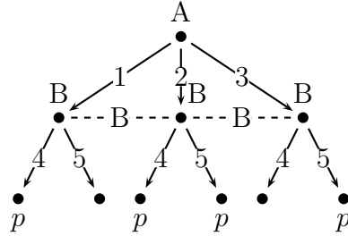
Figure 1.2: Game form G_2
