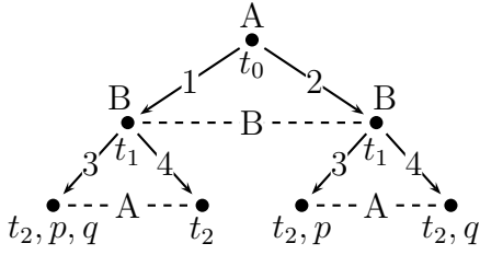
Figure 1.1: A simple game form G_1
