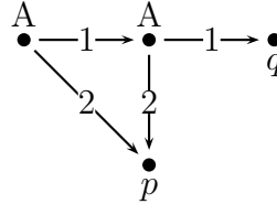
Figure 1.4: Block Pushing
