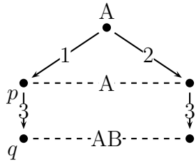
Figure 1.3: Imperfect Memory Game Form
